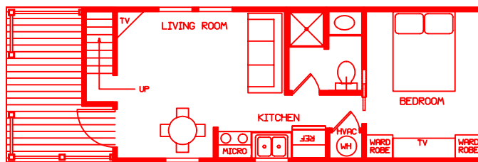
CUBBY CABIN STANDARD 12X36
