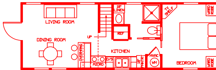
CUBBY CABIN STANDARD 12X34
